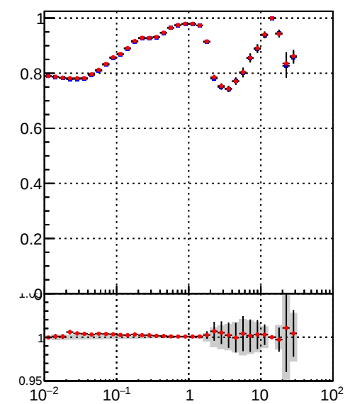
— /data2/legianni/BDT-vs-DNN/real-BDT/CMSSW_13_0_0_pre4/src/runrem/DQM_TT_mkFit_ — DQM_TT_mkFit_
