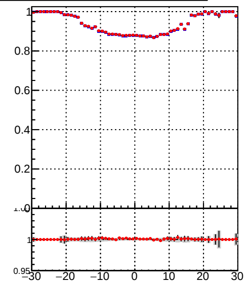
— /data2/legianni/BDT-vs-DNN/real-BDT/CMSSW_13_0_0_pre4/src/runrem/DQM_TT_mkFit_ — DQM_TT_mkFit_
