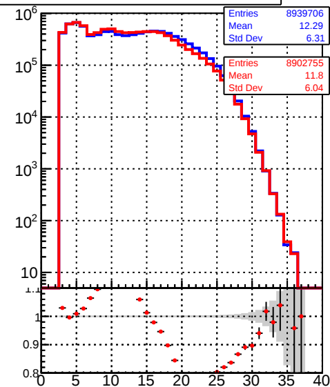
mean hit Legend: — /data2/legianni/BDT-vs-DNN/real-BDT/CMSSW_13_0_0_pre4/src/runrem/DQM_TT_mkFit_ — DQM_TT_mkFit_
