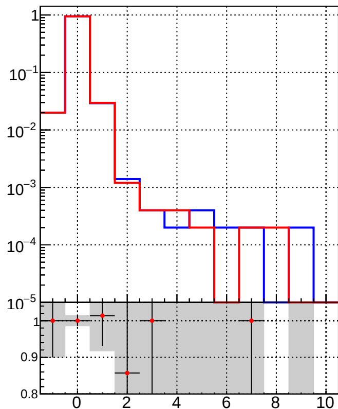
TruePVLocationIndexInRecoVertexCollection
