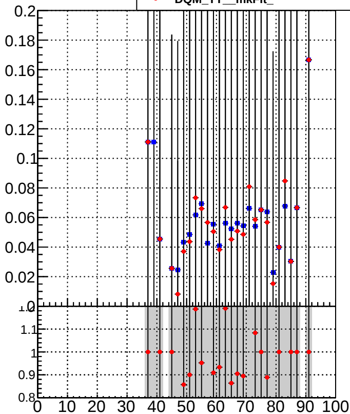
—■— /data2/legianni/BDT-vs-DNN/real-BDT/CMSSW_13_0_0_pre4/src/runrem/DQM_TT_mkFit_ —●— DQM_TT_mkFit_
