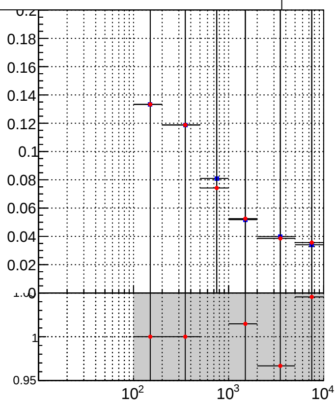
—■— /data2/legianni/BDT-vs-DNN/real-BDT/CMSSW_13_0_0_pre4/src/runrem/DQM_TT_mkFit_ —●— DQM_TT_mkFit_
