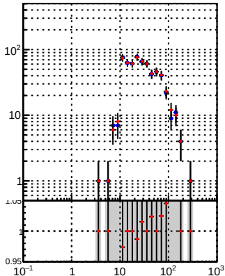
N of associated (recoToSim) tracks vs pT
