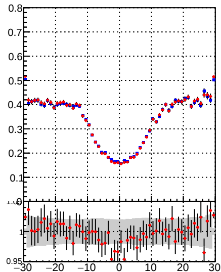
/data2/legianni/BDT-vs-DNN/real-BDT/CMSSW_13_0_0_pre4/src/runrem/DQM_TT_mkFit_ DQM_TT_mkFit_
