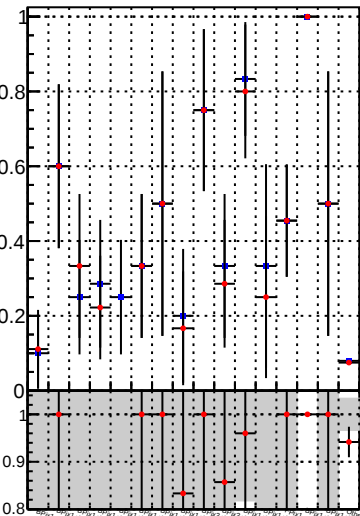
Fake rate vs. —•— /data2/legianni/BDT-vs-DNN/real-BDT/CMSSW_13_0_0_pre4/src/runrem/DQM_TT_mkFit_ —•— DQM_TT_mkFit_
