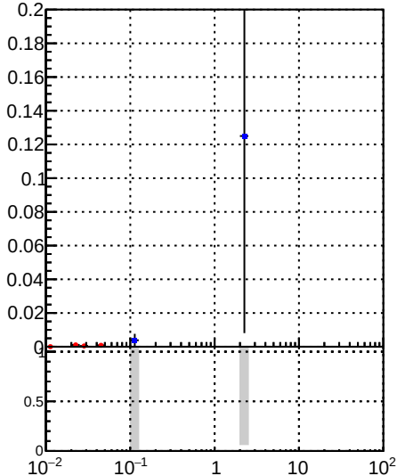
—●— /data2/legianni/BDT-vs-DNN/real-BDT/CMSSW_13_0_0_pre4/src/runrem/DQM_TT_mkFit_ —●— DQM_TT_mkFit_
