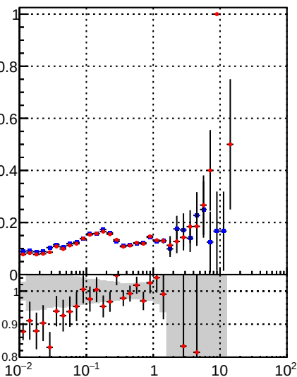
—•— /data2/legianni/BDT-vs-DNN/real-BDT/CMSSW_13_0_0_pre4/src/runrem/DQM_TT_mkFit_ —•— DQM_TT_mkFit_
