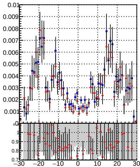
Fake rate vs d —●— /data2/legianni/BDT-vs-DNN/real-BDT/CMSSW_13_0_0_pre4/src/runrem/DQM_TT_mkFit_ —●— DQM_TT_mkFit_
