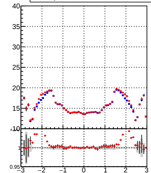
mean hit — /data2/legianni/BDT-vs-DNN/real-BDT/CMSSW_13_0_0_pre4/src/runrem/DQM_TT_mkFit_ — DQM_TT_mkFit_
