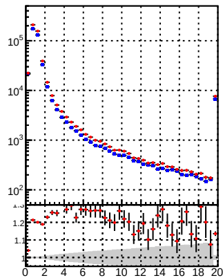
N of reco track vs. \chi^2 /data2/legianni/BDT-vs-DNN/real-BDT/CMSSW_13_0_0_pre4/src/runrem/DQM_TT_mkFit verSet
