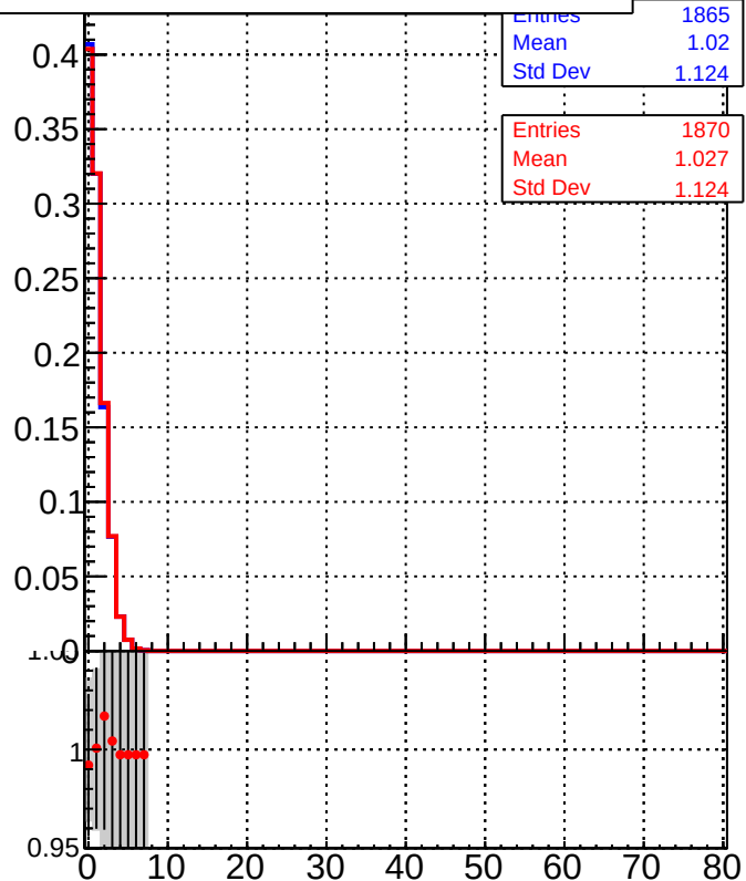
/data2/legianni/BDT-vs-DNN/real-BDT/CMSSW_13_0_0_pre4/src/runrem/DQM_TT_mkFit_ DQM_TT_mkFit_
