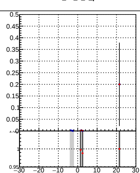
■ /data2/legianni/BDT-vs-DNN/real-BDT/CMSSW_13_0_0_pre4/src/runrem/DQM_TT_mkFit_ ● DQM_TT_mkFit_
