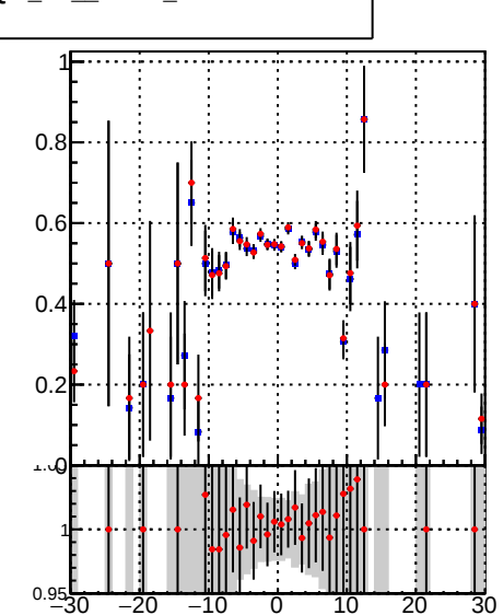
■ /data2/legianni/BDT-vs-DNN/real-BDT/CMSSW_13_0_0_pre4/src/runrem/DQM_TT_mkFit_ ● DQM_TT_mkFit_
