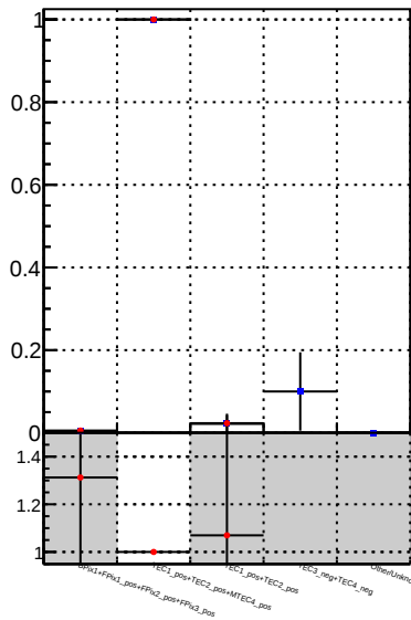
Fake rate vs. - /data2/legianni/BDT-vs-DNN/real-BDT/CMSSW_13_0_0_pre4/src/runrem/DQM_TT_mkFit_ - DQM_TT_mkFit
