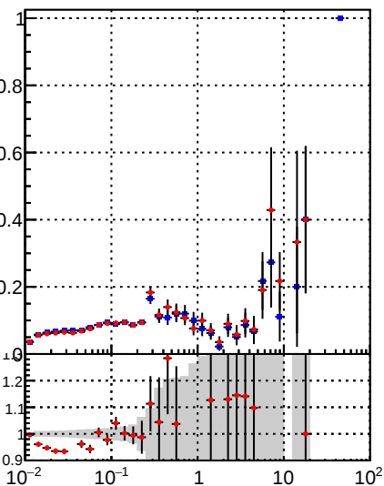
—●— /data2/legianni/BDT-vs-DNN/real-BDT/CMSSW_13_0_0_pre4/src/runrem/DQM_TT_mkFit_ —●— DQM_TT_mkFit_
