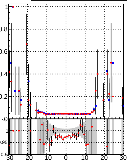
—●— /data2/legianni/BDT-vs-DNN/real-BDT/CMSSW_13_0_0_pre4/src/runrem/DQM_TT_mkFit_ —●— DQM_TT_mkFit_
