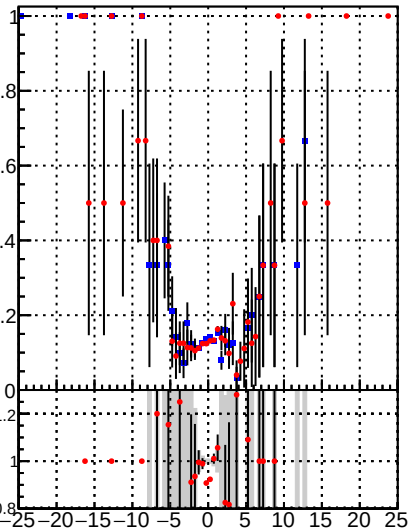
—●— /data2/legianni/BDT-vs-DNN/real-BDT/CMSSW_13_0_0_pre4/src/runrem/DQM_TT_mkFit_ —●— DQM_TT_mkFit_
