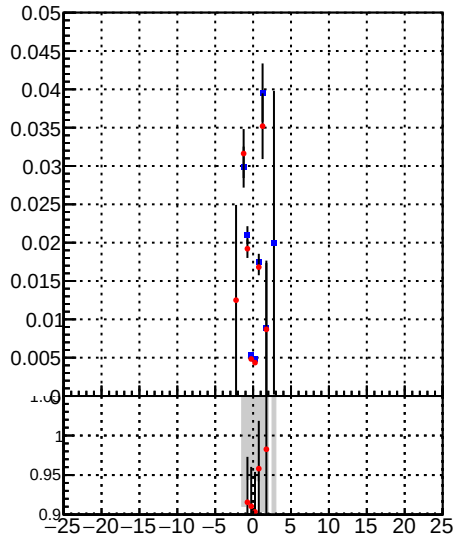
—●— /data2/legianni/BDT-vs-DNN/real-BDT/CMSSW_13_0_0_pre4/src/runrem/DQM_TT_mkFit_ —●— DQM_TT_mkFit_
