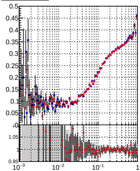
/data2/legianni/BDT-vs-DNN/real-BDT/CMSSW_13_0_0_pre4/src/runrem/DQM_TT_mkFit_ DQM_TT_mkFit_
