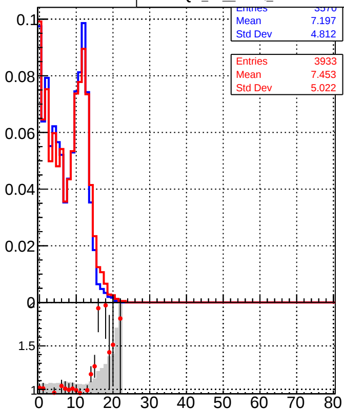
/data2/legianni/BDT-vs-DNN/real-BDT/CMSSW_13_0_0_pre4/src/runrem/DQM_TT_mkFit DQM_TT_mkFit
