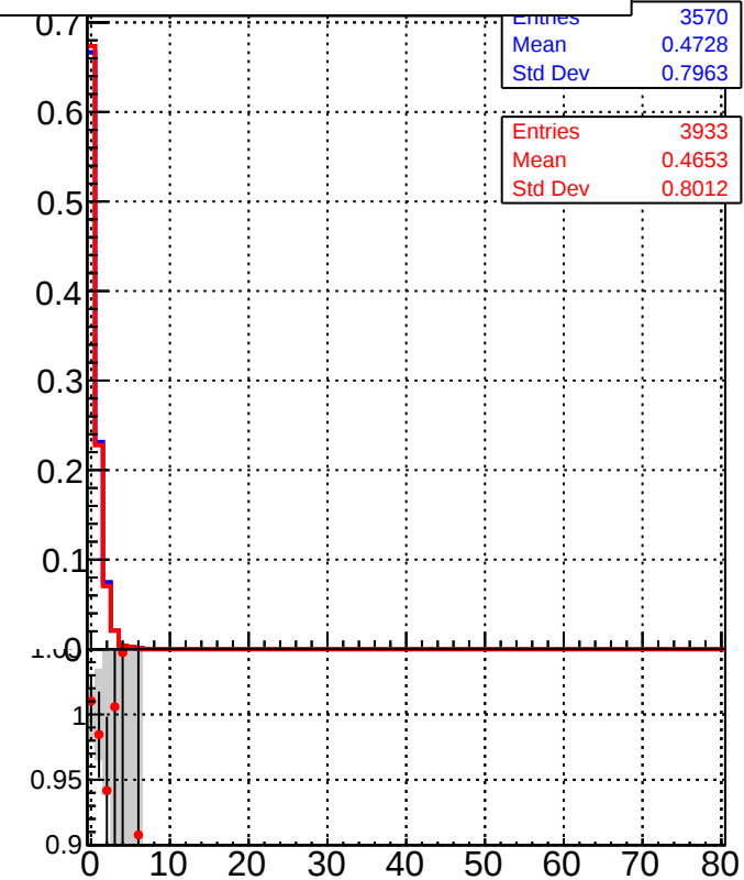
/data2/legianni/BDT-vs-DNN/real-BDT/CMSSW_13_0_0_pre4/src/runrem/DQM_TT_mkFit DQM_TT_mkFit
