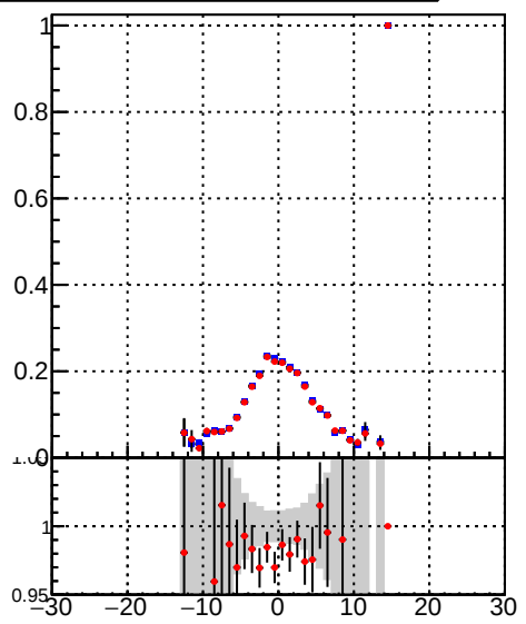
Efficiency vs. sim PV z Legend: — /data2/legianni/BDT-vs-DNN/real-BDT/CMSSW_13_0_0_pre4/src/runrem/DQM_TT_mkFit_ — DQM_TT_mkFit_
