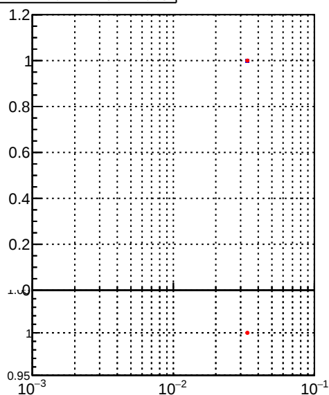
Efficiency vs \Delta R(\text{track}, \text{jet})
