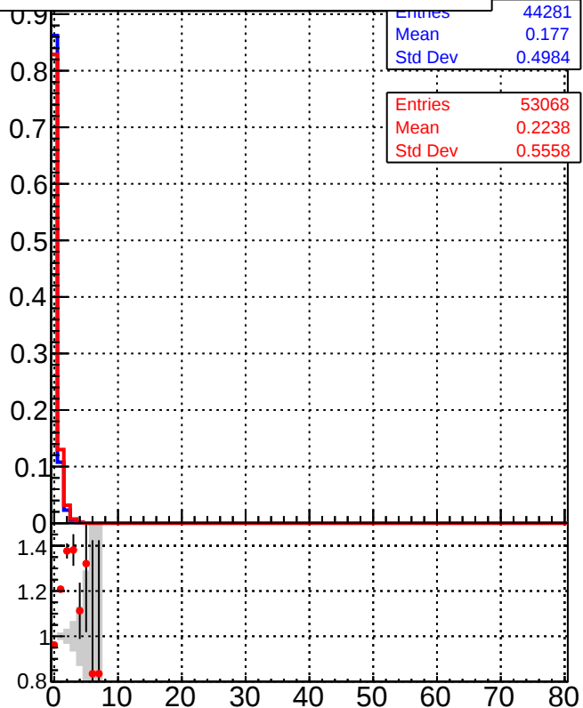
Legend for bottom row plots: ■ /data2/legianni/BDT-vs-DNN/real-BDT/CMSSW_13_0_0_pre4/src/runrem/DQM_TT_mkFit_ ● DQM_TT_mkFit_
