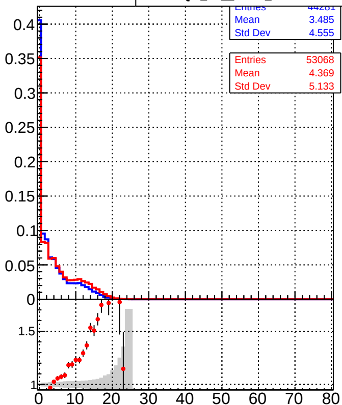
Legend for bottom row plots: ■ /data2/legianni/BDT-vs-DNN/real-BDT/CMSSW_13_0_0_pre4/src/runrem/DQM_TT_mkFit_ ● DQM_TT_mkFit_
