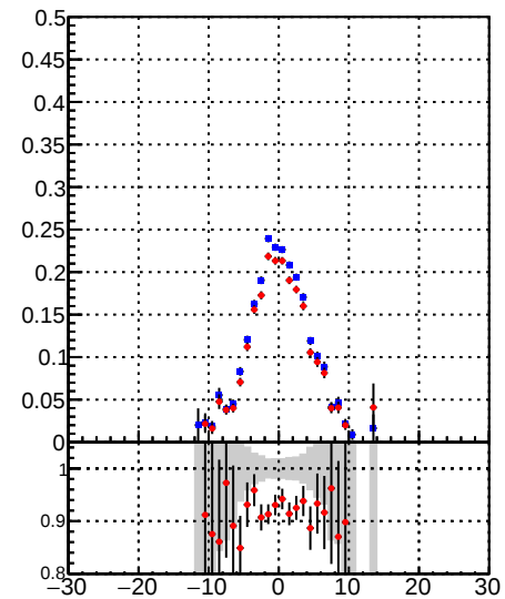
Fake rate vs d — /data2/legianni/BDT-vs-DNN/real-BDT/CMSSW_13_0_0_pre4/src/runrem/DQM_TT_mkFit_ — DQM_TT_mkFit_
