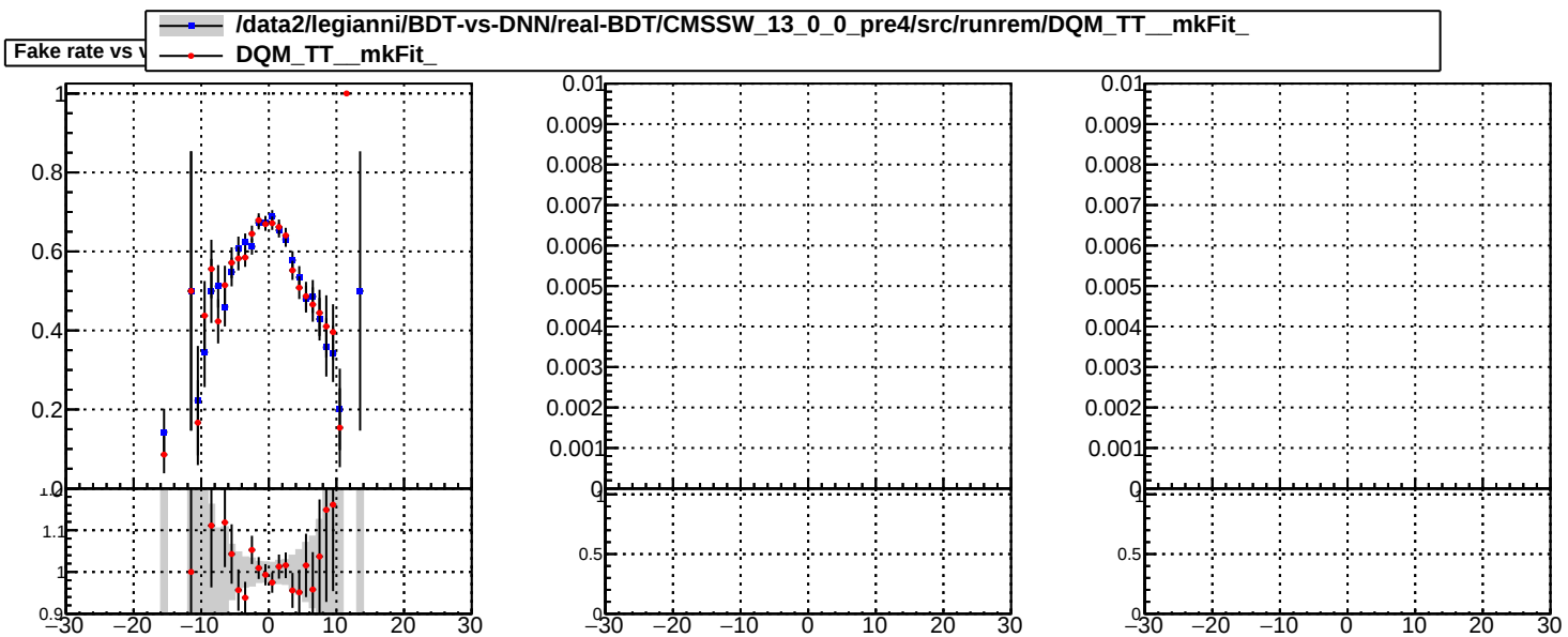
Fake rate vs. sim PV z
