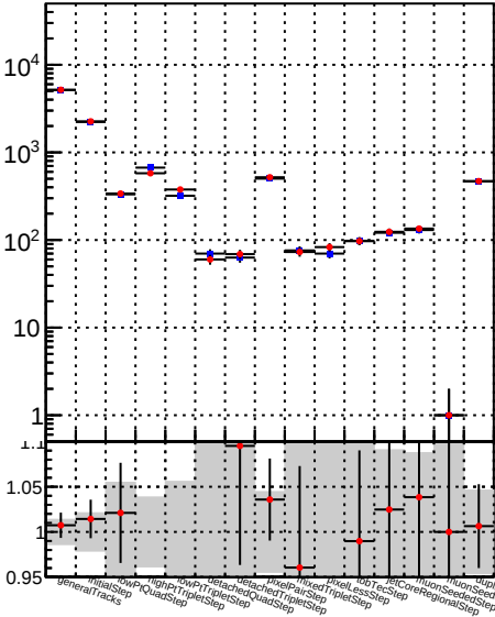
Number —●— DQM_TT_mkFit
