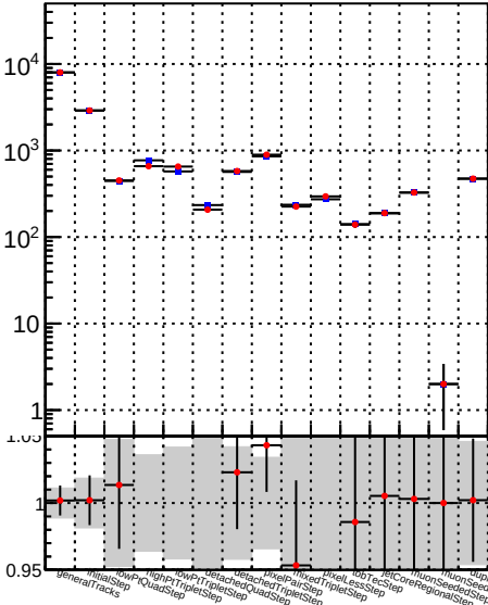
Number —●— DQM_TT_mkFit
