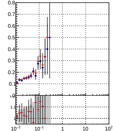
—●— /data2/legianni/BDT-vs-DNN/real-BDT/CMSSW_13_0_0_pre4/src/runrem/DQM_TT_mkFit_ —●— DQM_TT_mkFit_
