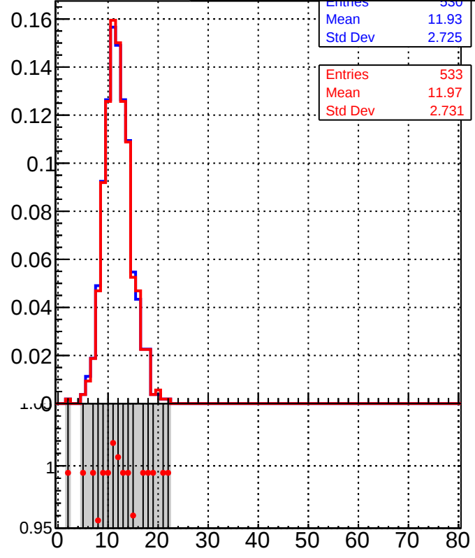
/data2/legianni/BDT-vs-DNN/real-BDT/CMSSW_13_0_0_pre4/src/runrem/DQM_TT_mkFit_ DQM_TT_mkFit_
