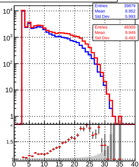
mean hit — /data2/legianni/BDT-vs-DNN/real-BDT/CMSSW_13_0_0_pre4/src/runrem/DQM_TT_mkFit_ — DQM_TT_mkFit_
