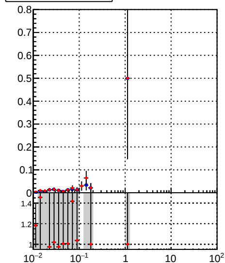
—●— /data2/legianni/BDT-vs-DNN/real-BDT/CMSSW_13_0_0_pre4/src/runrem/DQM_TT_mkFit_ —●— DQM_TT_mkFit_
