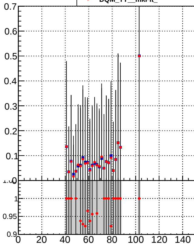
—■— /data2/legianni/BDT-vs-DNN/real-BDT/CMSSW_13_0_0_pre4/src/runrem/DQM_TT_mkFit_ —●— DQM_TT_mkFit_
