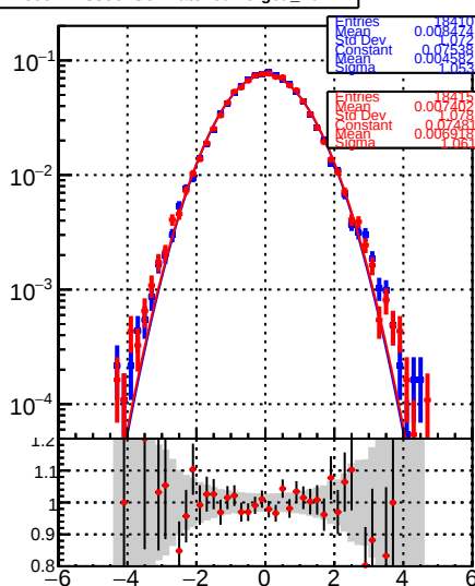
RecoAllAssoc2GenMatchedMerged_PulIX
