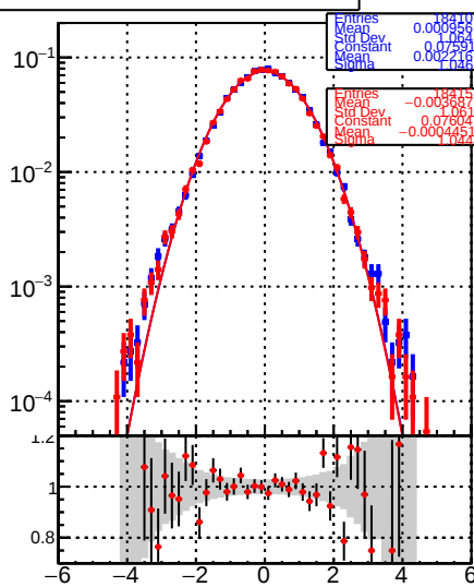
RecoAllAssoc2GenMatchedMerged_PulIZ
