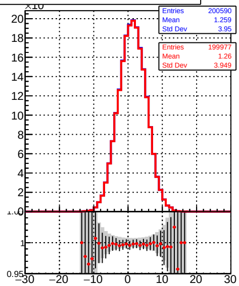
Recons /data2/legianni/BDT-vs-DNN/real-BDT/CMSSW_13_0_0_pre4/src/runrem/DQM_TT_mkFit_
