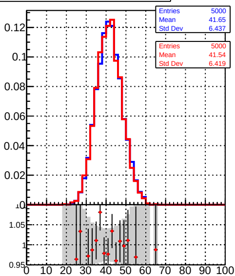
ReconstructedAllAssoc2Gen_NumVertices
