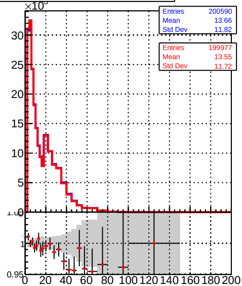
ReconstructedAllAssoc2Gen_NumTracks
