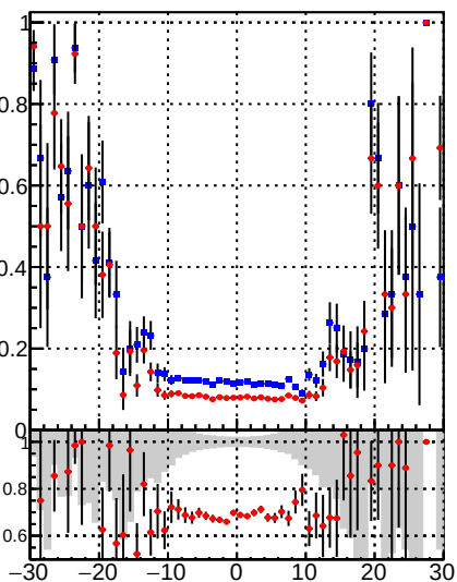
Fake rate vs d —•— /data2/legianni/BDT-vs-DNN/real-BDT/CMSSW_13_0_0_pre4/src/runrem/DQM_TT_mkFit_ —•— DQM_TT_mkFit_
