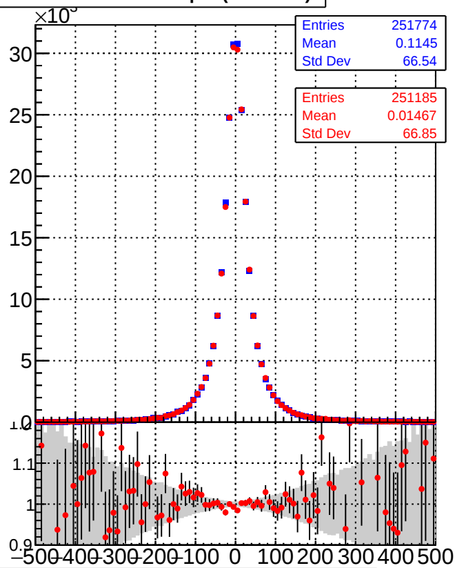
X distance from BeamSpot (other Vtx)
