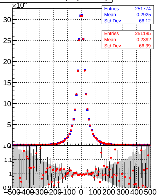
Y distance from BeamSpot (other Vtx)
