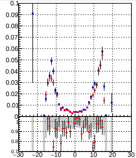
—●— /data2/legianni/BDT-vs-DNN/real-BDT/CMSSW_13_0_0_pre4/src/runrem/DQM_TT_mkFit_ —+— DQM_TT_mkFit_
