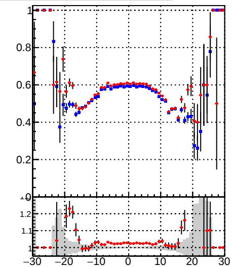
—●— /data2/legianni/BDT-vs-DNN/real-BDT/CMSSW_13_0_0_pre4/src/runrem/DQM_TT_mkFit_ —+— DQM_TT_mkFit_
