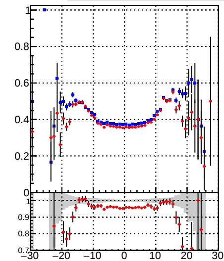
—●— /data2/legianni/BDT-vs-DNN/real-BDT/CMSSW_13_0_0_pre4/src/runrem/DQM_TT_mkFit_ —+— DQM_TT_mkFit_
