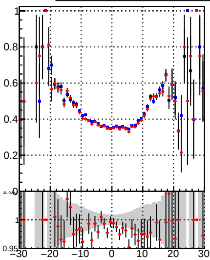
—●— /data2/legianni/BDT-vs-DNN/real-BDT/CMSSW_13_0_0_pre4/src/runrem/DQM_TT_mkFit_ —+— DQM_TT_mkFit_
