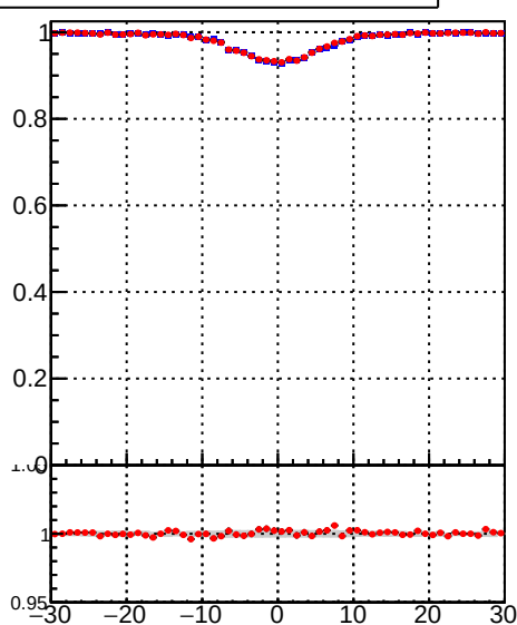
Efficiency vs vertpos - /data2/legianni/BDT-vs-DNN/real-BDT/CMSSW_13_0_0_pre4/src/runrem/DQM_TT_mkFit_ - DQM_TT_mkFit_
