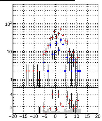
N of associated (recoToSim) lepton tracks vs. sim PV z
