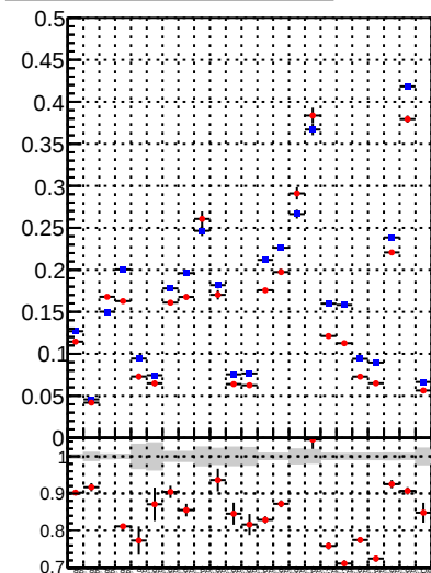
— /data2/legianni/BDT-vs-DNN/real-BDT/CMSSW_13_0_0_pre4/src/runrem/DQM_TT_mkFit_ — DQM_TT_mkFit
