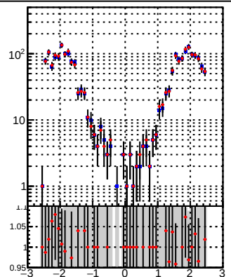
Legend: - Blue line: /data2/legianni/BDT-vs-DNN/real-BDT/CMSSW_13_0_0_pre4/src/runrem/DQM_TT_mkFit_ - Red line: DQM_TT_mkFit_ - Green line: N of reco track vs eta
