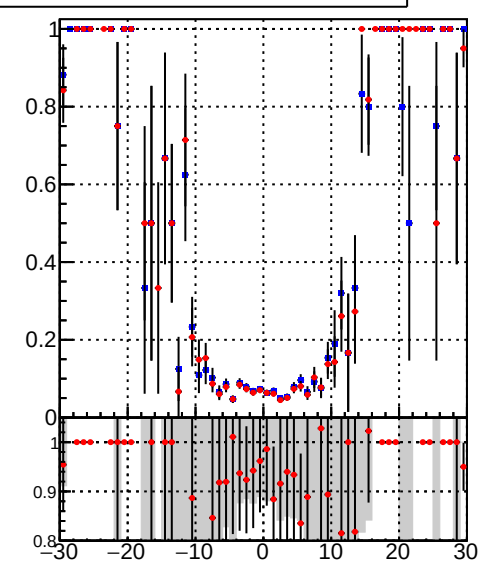
Efficiency vs vertpos - /data2/legianni/BDT-vs-DNN/real-BDT/CMSSW_13_0_0_pre4/src/runrem/DQM_TT_mkFit_ - DQM_TT_mkFit_
