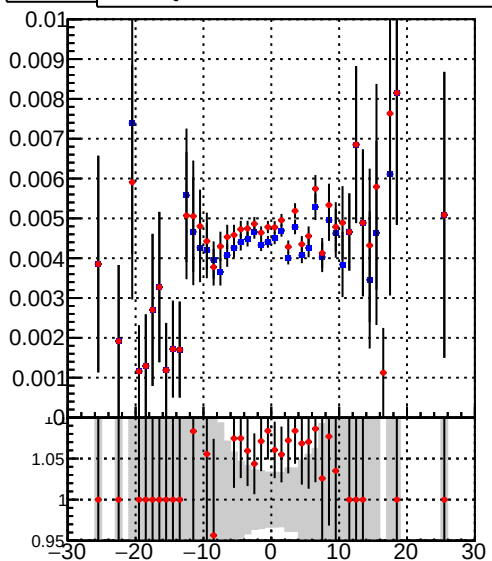
Efficiency vs vertpos - /data2/legianni/BDT-vs-DNN/real-BDT/CMSSW_13_0_0_pre4/src/runrem/DQM_TT_mkFit_ - DQM_TT_mkFit_
