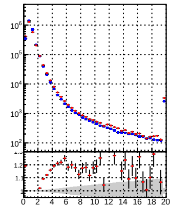
N of reco track vs. \chi^2 /data2/legianni/BDT-vs-DNN/real-BDT/CMSSW_13_0_0_pre4/src/runrem/DQM_TT_mkFit
