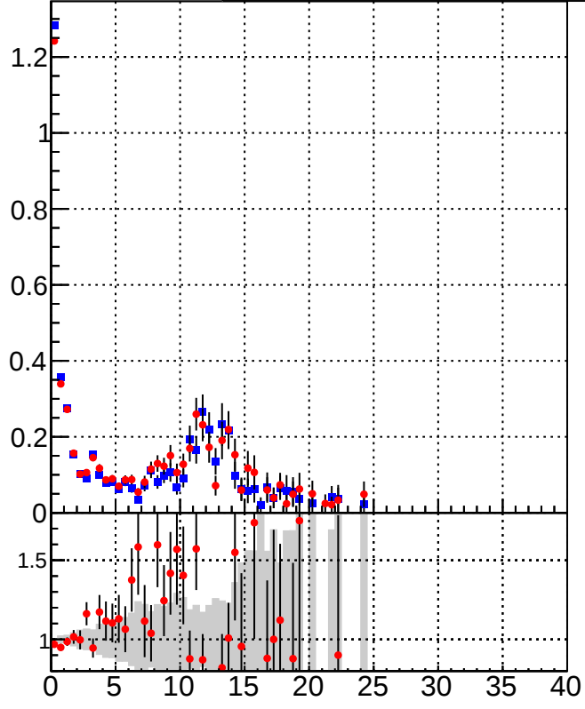
K_S^0 tracking fake rate vs p_T and \eta Legend: \square /data2/legianni/BDT-vs-DNN/real-BDT/CMSSW_13_0_0_pre4/src/runrem/DQM_TT_mkFit_ \circ DQM_TT_mkFit_
