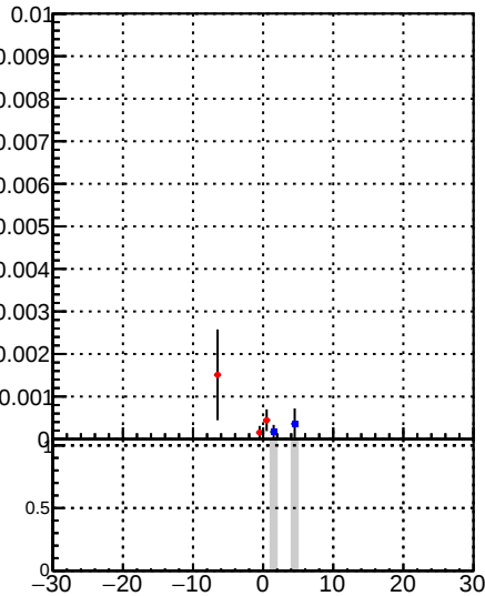
/data2/legianni/BDT-vs-DNN/real-BDT/CMSSW_13_0_0_pre4/src/runrem/DQM_TT_mkFit_ DQM_TT_mkFit_
