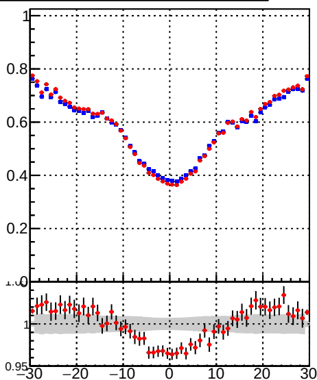
— /data2/legianni/BDT-vs-DNN/real-BDT/CMSSW_13_0_0_pre4/src/runrem/DQM_TT_mkFit_ — DQM_TT_mkFit_
