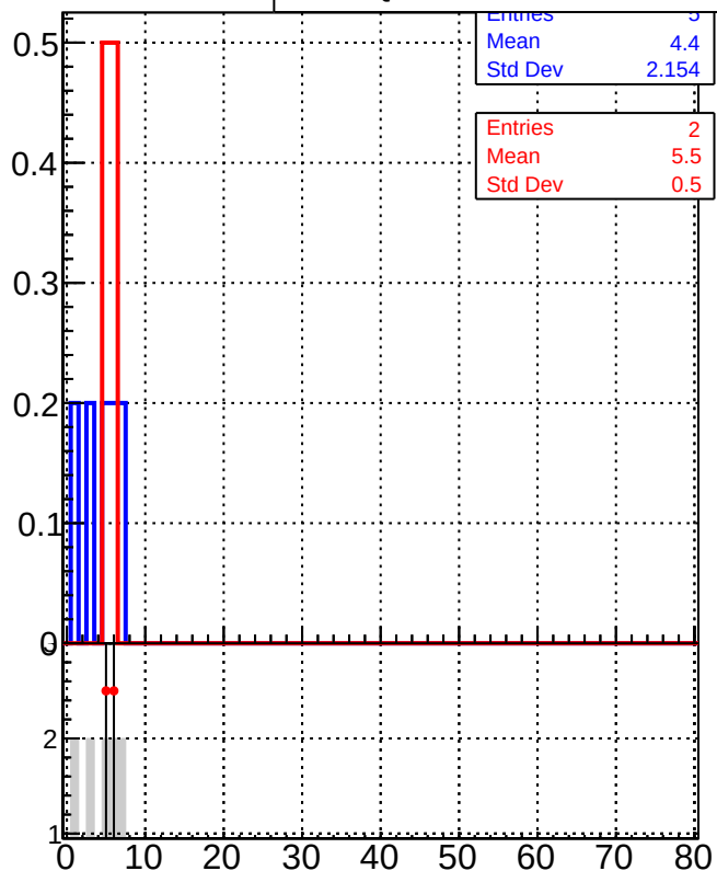
Legend: /data2/legianni/BDT-vs-DNN/real-BDT/CMSSW_13_0_0_pre4/src/runrem/DQM_TT_mkFit
