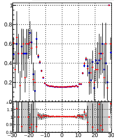
—•— /data2/legianni/BDT-vs-DNN/real-BDT/CMSSW_13_0_0_pre4/src/runrem/DQM_TT_mkFit_ —•— DQM_TT_mkFit_ Fake rate vs v
