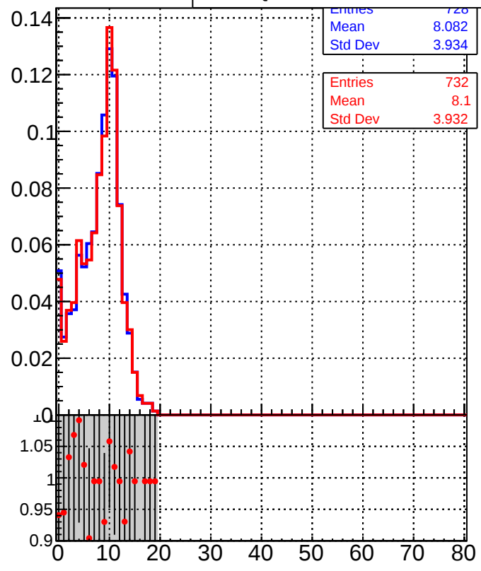
/data2/legianni/BDT-vs-DNN/real-BDT/CMSSW_13_0_0_pre4/src/runrem/DQM_TT_mkFit_
