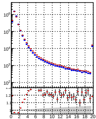
N of reco track vs. \chi^2 for /data2/legianni/BDT-vs-DNN/real-BDT/CMSSW_13_0_0_pre4/src/runrem/DQM_TT_mkFit
