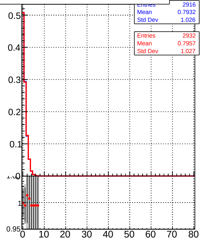
/data2/legianni/BDT-vs-DNN/real-BDT/CMSSW_13_0_0_pre4/src/runrem/DQM_TT_mkFit
